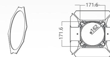
Accessory holder (2440010251)
