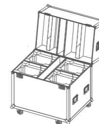
Flight Case (1320400177)
