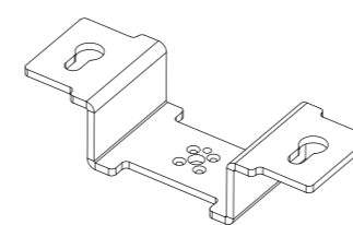
壁挂支架 (2440120199)
