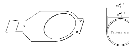
Gobo holder (2440010803)
