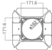
挡光叶 (2440010210)
