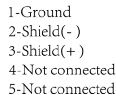
XLR mounting-plugs
